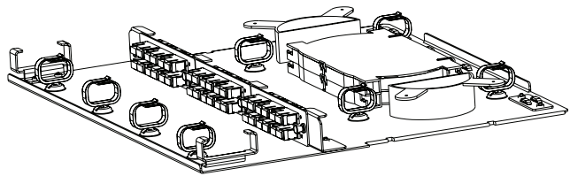
Splicing drawer of 1U Height with 3-slot Use to house 3pcs of Size-B Faceplate (refer to Page 90)
