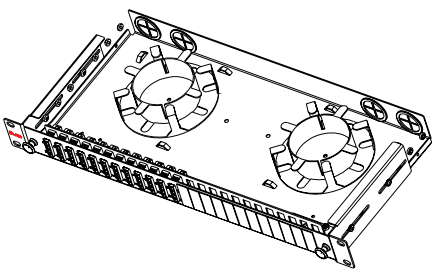
Example of D200, LC, 48-Fiber, Patching, OM2 P/N: R200P1G-4CM2
