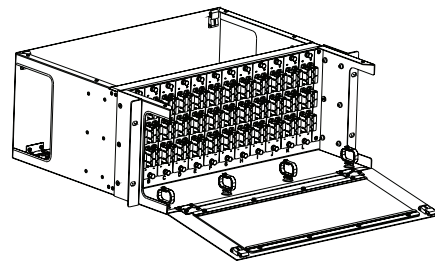
4U Fixed Type Enclosure (Vertical Style )
