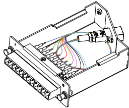
12-Fiber Cassette with 1x12F MPO interface
