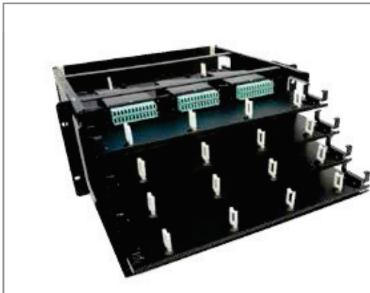
Example of Drawer Type Enclosure in 4U, preloaded with 4pcs of M3A-Drawer
