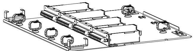
Plug-and-play drawer use to house 4pcs of Size-B Cassette (refer to Page 86)
