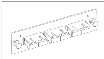
Size-B Faceplate: 32(H) x 120(W)mm
