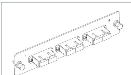
Size-A Faceplate: 32(H) x 150(W)mm
